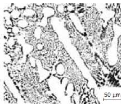
d) SnPb10
